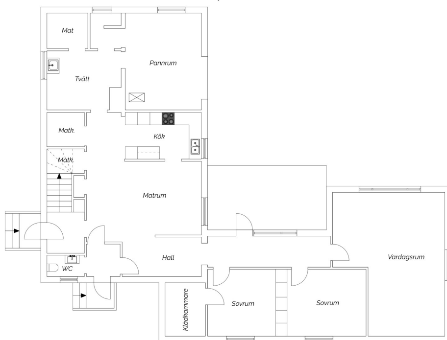
Bottenplan
