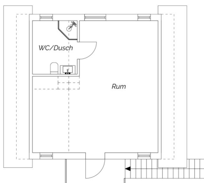
Ovanplan garage
